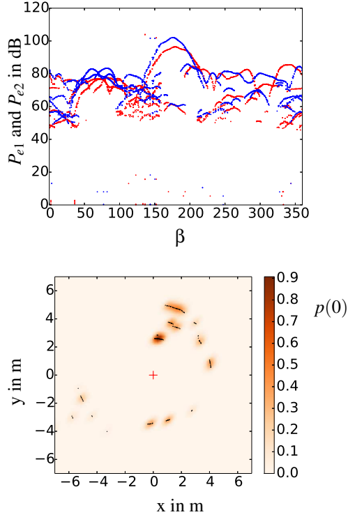
Figure 6: Above: This diagram depicts the power at the receiver antennas P_{e1} and P_{e2} during a 360^\circ scan. The non-point target effect does not effect the results. The main error influence is caused by the low resolution and the wide beam size of the radar sensor. An angle estimation of objects through the ASR in a traditional way is impossible, because of the non-uniform distribution of the power values. Below: This diagram presents a 2D scan of our office environment via the ASR technique. The red cross shows the location of the sensor unit.
