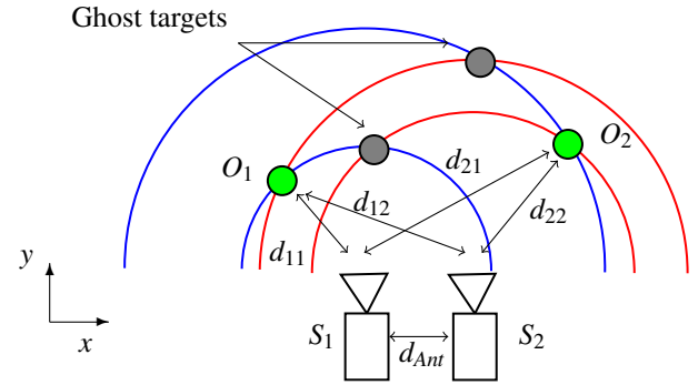
Figure 1: The position of objects O can be estimated via the distances d , which are measured from different sensors. Ghost targets represent a geometrical ambiguity.
