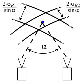
Figure 3: Area of ambiguity, which is caused by the two rms-errors \sigma_{R1} and \sigma_{R2} .
